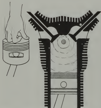
FIGURE 10-32. Normal combustion within a cylinder.
